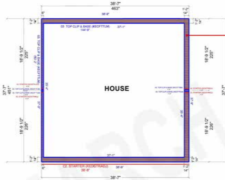
REFLECTED CEILING PLAN UPPER LEVEL: HOUSE SOFFIT DETAIL "D" SCALE: 1/4" = 1FT
