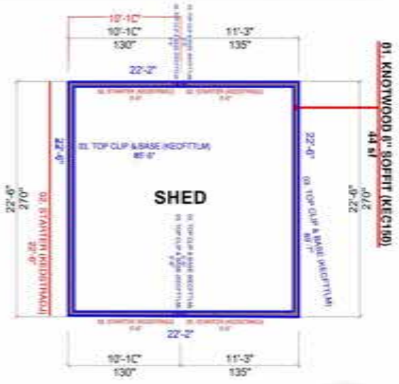
REFLECTED CEILING PLAN MAIN LEVEL: SHED DETAIL "A" SCALE: 1/4" = 1FT
