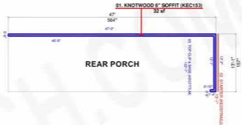
REFLECTED CEILING PLAN MAIN LEVEL: REAR PORCH SOFFIT DETAIL "B" SCALE: 1/4" = 1FT
