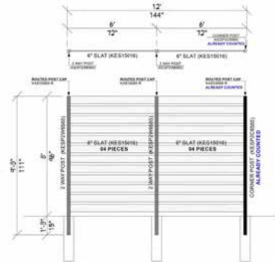
12' FENCE DETAIL
