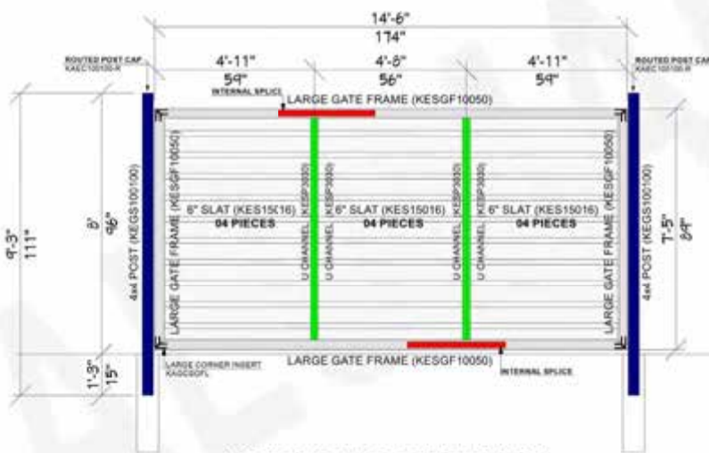
14'6" SLIDING GATE DETAIL
