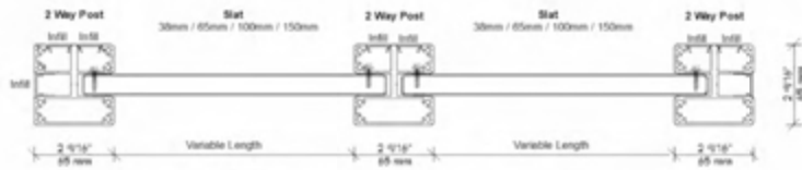
STANDARD SCREEN ASSEMBLY
